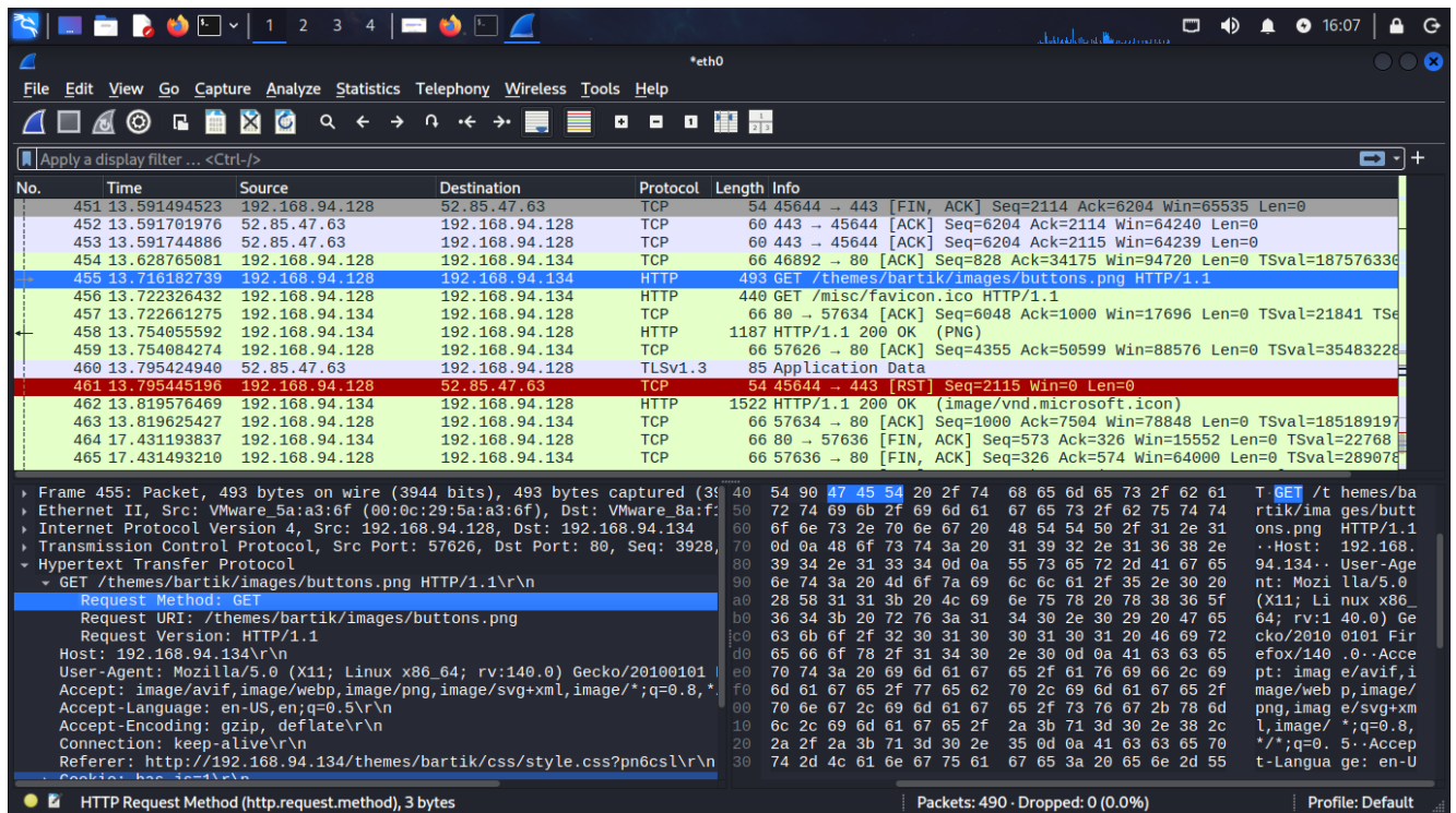
Figure 2: Wireshark capture showing HTTP traffic between Kali Linux and DC-1
